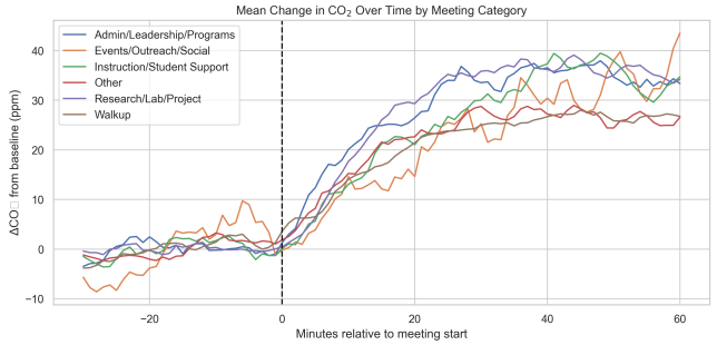
Figure 5: Mean CO 2 Pattern Over Time. Values are normalized to the 30-minute pre-meeting baseline.
